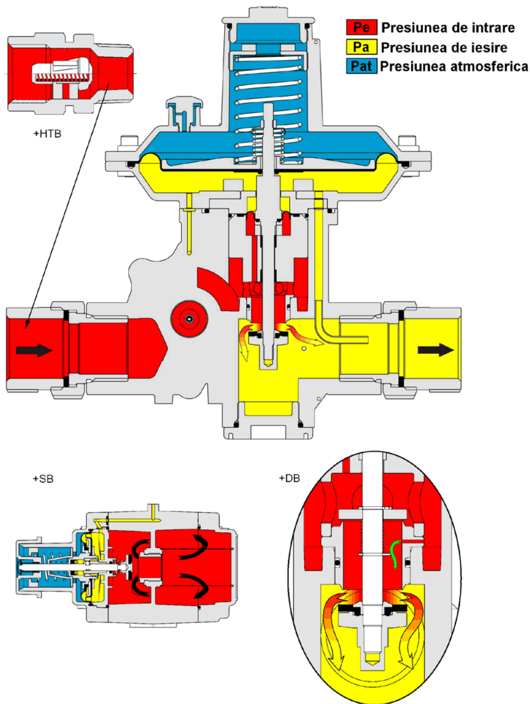
Figura 1 – Regulatorul RTG 25
